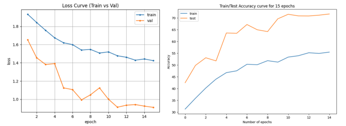
Fig. 5. CNN Accuracy and Loss curves for CIFAR10
