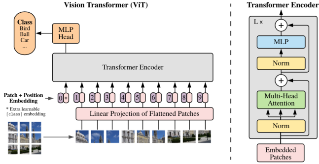
Fig. 2. ViT High level Architecture
