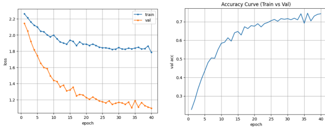
Fig. 6. Vision Transformer Accuracy and Loss curves for CIFAR10
