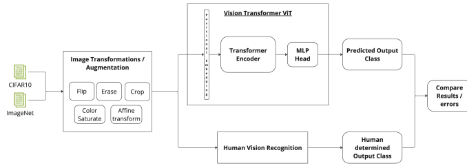
Fig. 3. A rough design of the Computational Model
